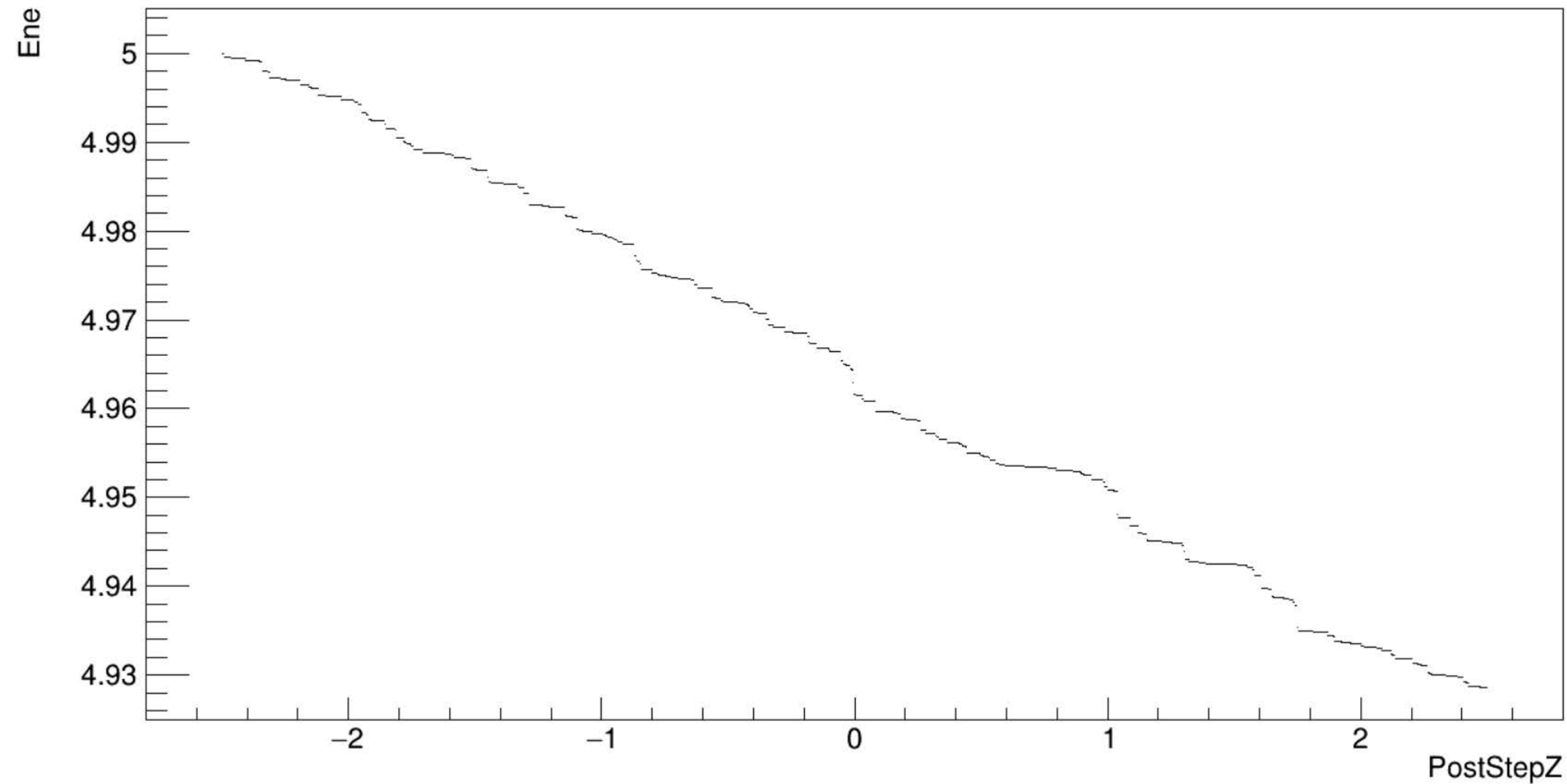
Ene:PostStepZ {EventNumber == 1500}
