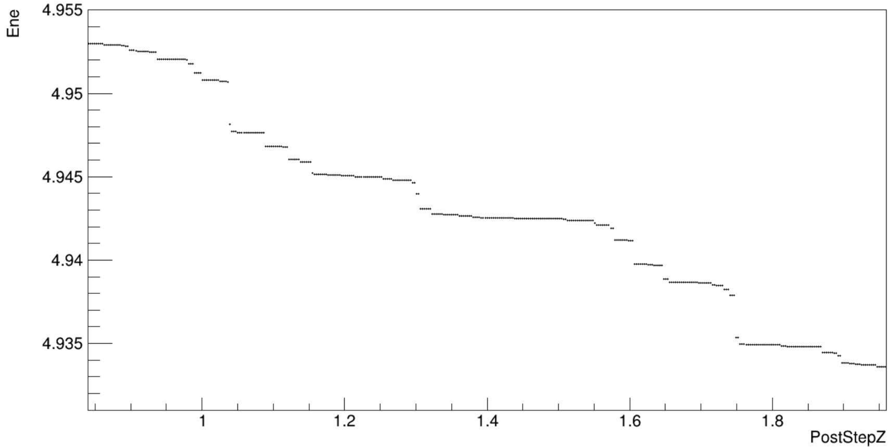
Ene:PostStepZ {EventNumber == 1500}
