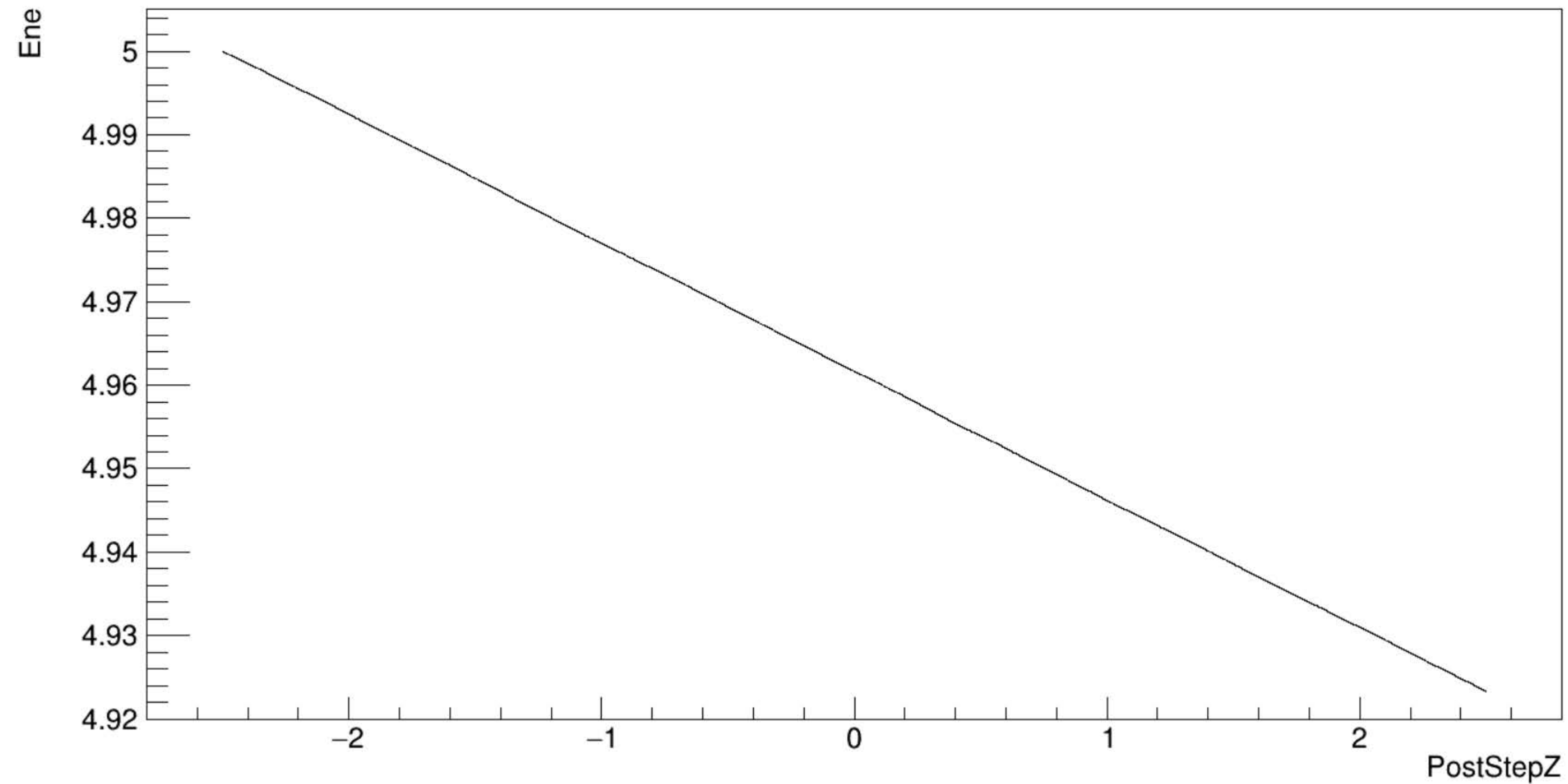
Ene:PostStepZ {EventNumber == 1500}
