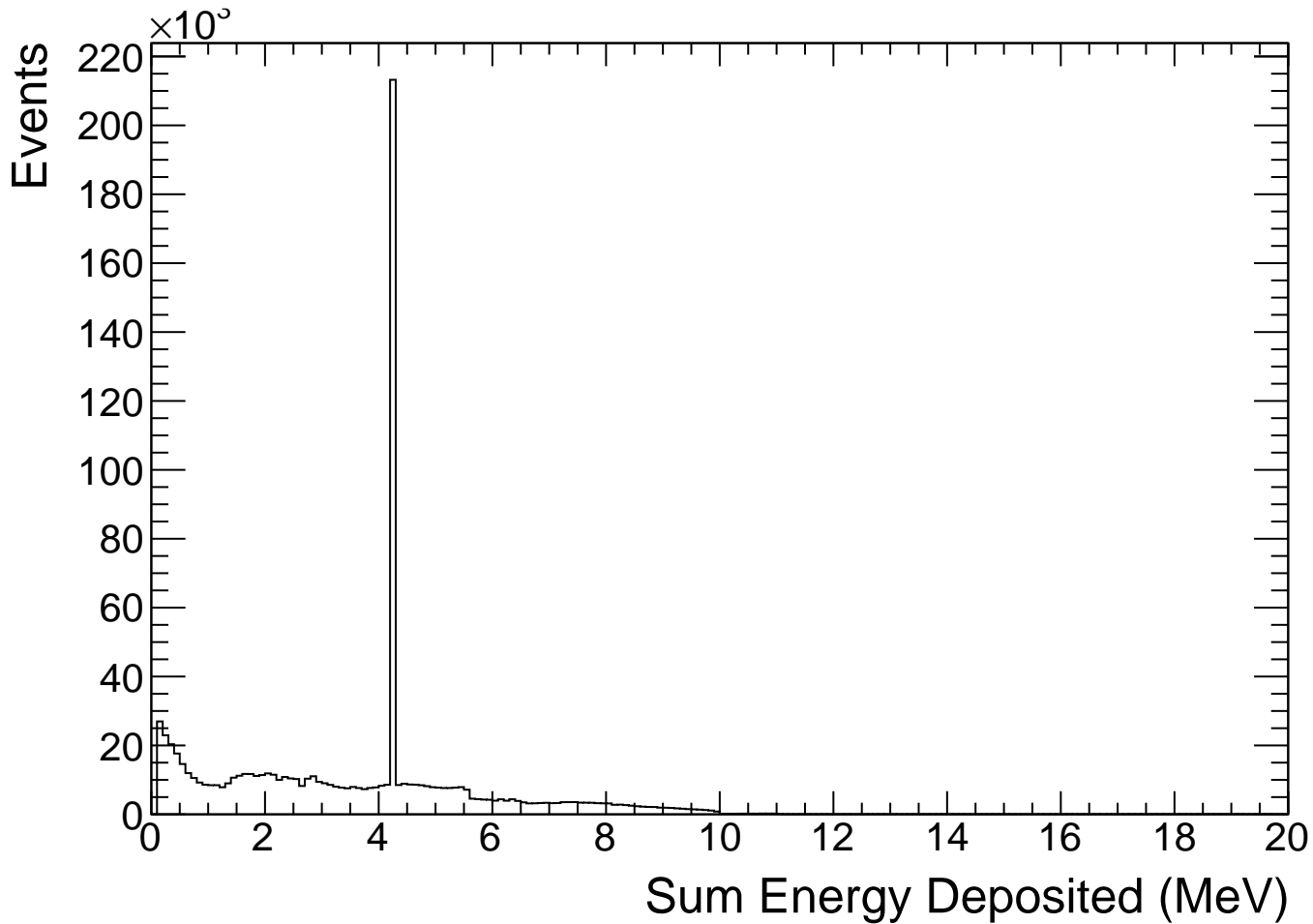
Energy Deposited 10 Mev Neutron From all Secondary Particles
