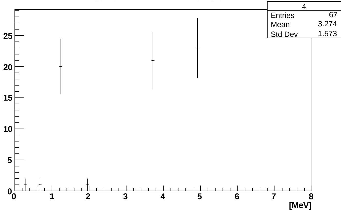
energy spectrum of emerging gamma
